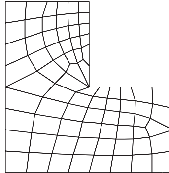
Fig. 32. 1st. Adaptive step - (REP)
