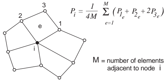
Fig. 25. Quadrilateral element mesh smoothing procedure. The position of each internal node is adjusted to lie at the centroid of the polygon formed by its adjacent elements
