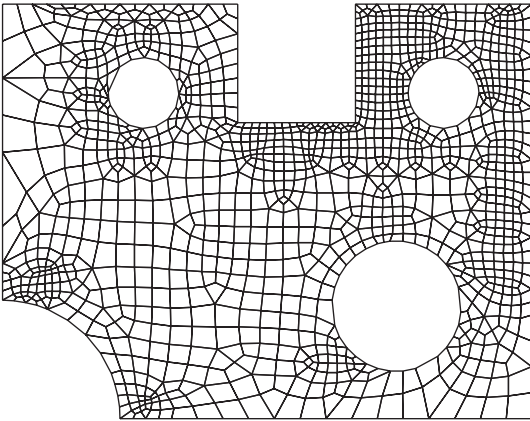
Fig. 50. 1st. Self-adaptive step (Q4)
