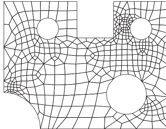
Fig. 53. 1st. Self-adaptive step (Q8)
