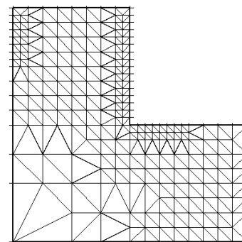
Fig. 13. Resulting mesh
