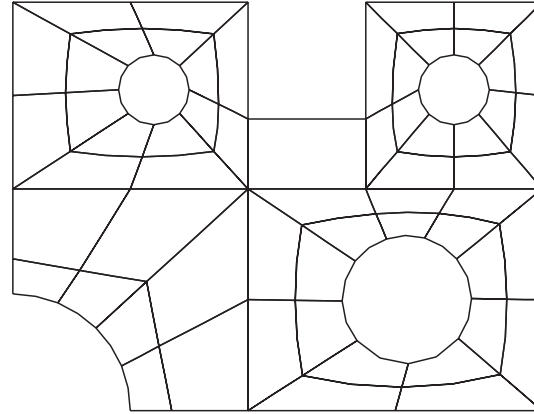
Fig. 52. Initial finite element mesh (Q8)
