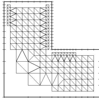
Fig. 12. Interior mesh
