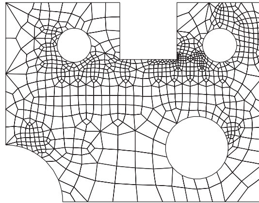
Fig. 54. 2nd. Self-adaptive step (Q8)
